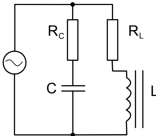
Drawing 23: Parallel Resonant Circuit
